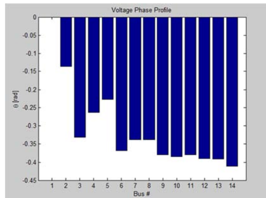
Figure 6. Voltage Phase Profile of IEEE 14 bus test.
