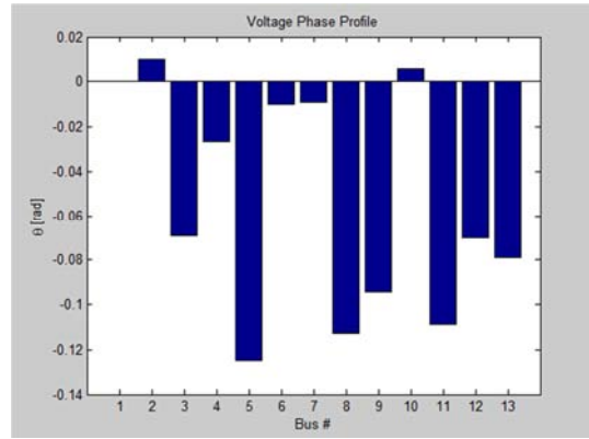
Figure 5. Voltage phase Profile of Northern Nigeria.
