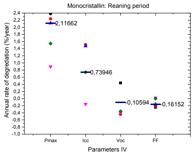
Figure 2. Degradation of I-V parameters (Isc, Voc & FF) for PV Monocrystalline Module technology.
