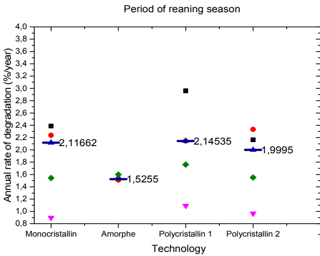
Figure 1. Influence of PV module technology on the degradation of maximum power.
