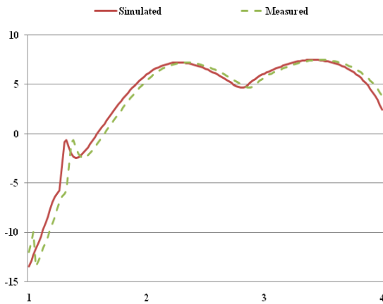
Figure 10. Gain Vs frequency of proposed antenna shown in Figure 1.
