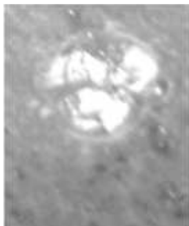
Fig. (11). Lepidocyclina (Nephrolepidina) tournoueri Unit (VIII),sample(26) Qarah chauq Dagh section, Azkand Formation. oriented section (35X)
