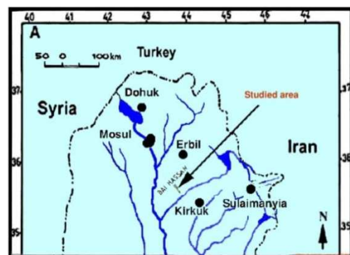
Fig (1). Location map of the Studied Well.
