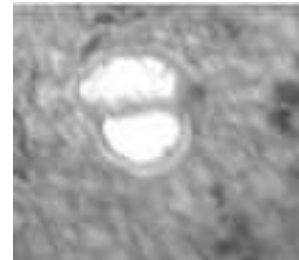
Fig. (6). Lepidocyclus ( Nephrolepidina ) morgani , Unit (IV), sample(23) Bai-Hassan well-4 section, Baba Formation. oriented section (30X)
