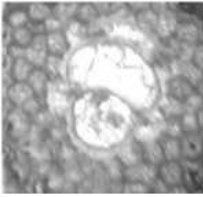
Fig. (8). Lepidocyclina (Nephrolepidina) morgani Unit(VII),sample (18),Qarah chauq Dagh section, Azkand Formation. oriented section (40X)
