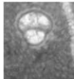
Fig. (7). Lepidocyclus ( Nephrolepidina ) morgani , Unit (II), sample(22) Bai-Hassan well-4 section, Baba Formation. oriented section (35X)
