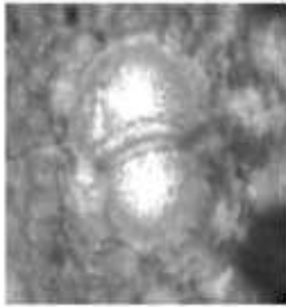
Fig. (9). Lepidocyclina (Nephrolepidina) morgani ,Unit (VII),sample(18) Qarah chauq Dagh section, Azkand Formation. oriented section (30X)
