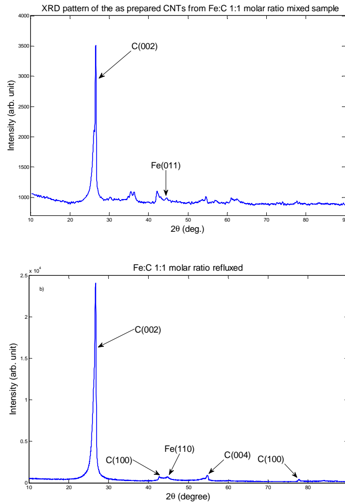
Fig. 2. XRD pattern of CNTs from Fe:C1:1 molar ratio as prepared (a) and post purification (b) with their corresponding planes[25].
