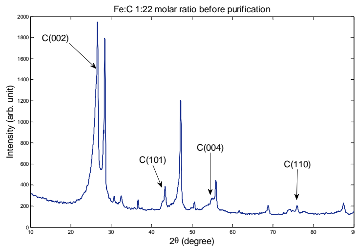
Fig. 3. XRD pattern of as prepared CNTs from C:Fe 22:1. The diffraction peaks emerged at 26.42° corresponds to C(002) plane, 43.43° corresponds to C(101) and so on have resemblance with that of graphite. The remaining peaks reveal the existence of any other kind of ingredient including iron nano particles in the sample.
