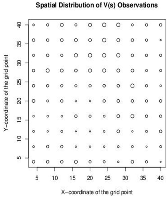
(c) A plot of V(s) with an exponential variogram
