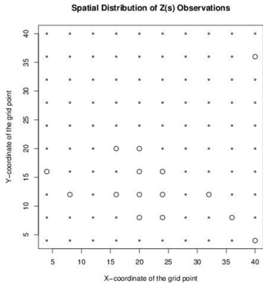
(f) The plot of generated spatial correlated binary data where V(s) has spherical variogram
