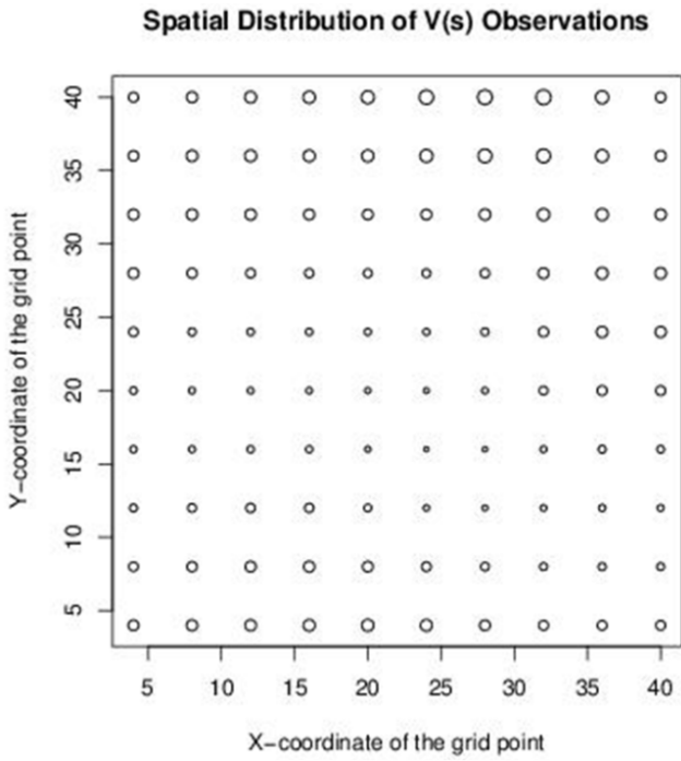
(a) A plot of V(s) with Gaussian variogram
