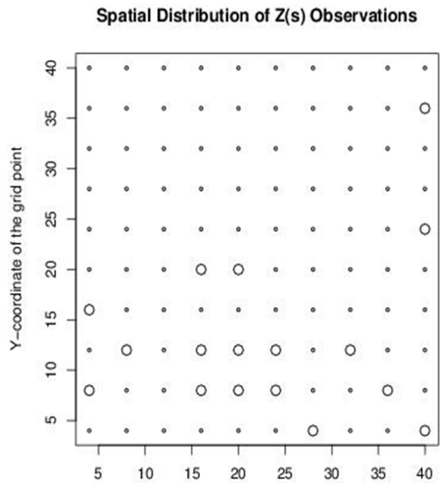
(d) The plot of generated spatial correlated binary data where V(s) has an exponential variogram
