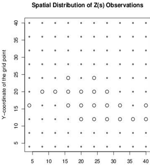
(b) The plot of generated spatial correlated binary data where V(s) has a Gaussian variogram
