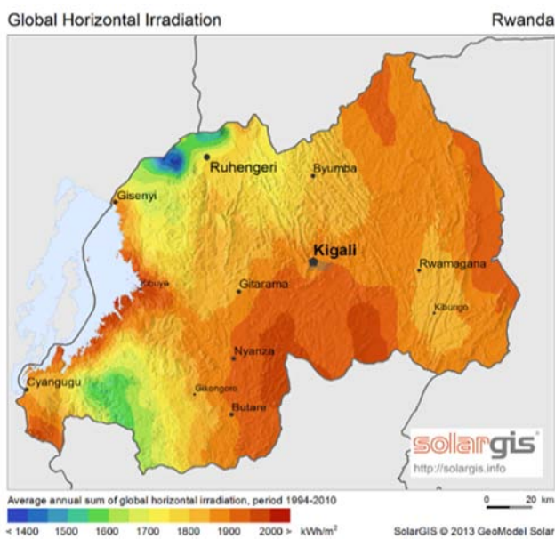
Figure 1. Rwanda global horizontal irradiation. Source: Solargis [27].
