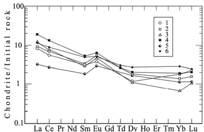
Figure 7. Distribution REE in ore bearing and host rocks of RLH intrusion Pansky Tundra. 1-ma254g - gabbronorite, 2-ma251r - ore bearing anorthosite, 3- ys228r - ore bearing anorthosite, 4-yk221r - ore bearing anorthosite, 5-yk216g - gabbronorite, 6-yk217 - gabbronorite. Positive Eu anomaly is clear visible for ore bearing anorthosites.
