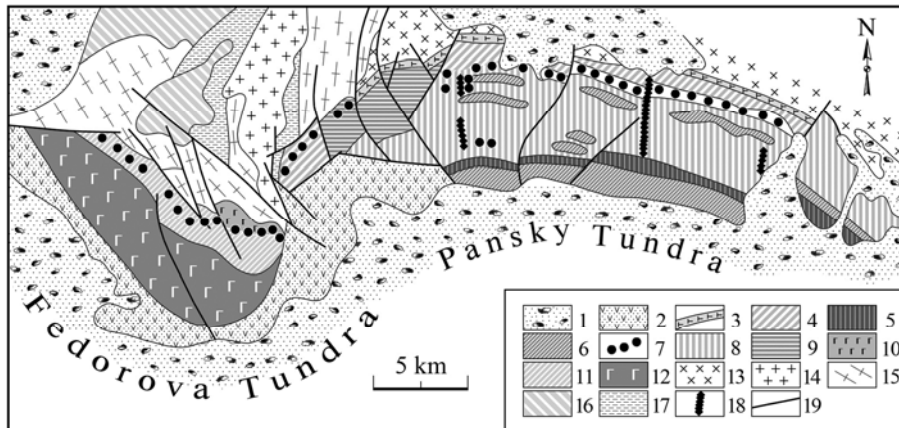
Figure 1. Scheme geological construction layered intrusions Fedorova and Pansky Tundra. 1- Modern deposits, 2-Paleoproterozoic sedimentary-volcanic rocks of Imandra–Varsuga structure. Rocks of Fedorova-Pansky intrusion: 3-gabbro, norites, gabbronorites of lower boundary zone, 4-gabbronorites lower zone, 5- upper rhythmic layered horizon, 6-gabbronorites stripped and trachitoidal upper zone, 7- lower rhythmic layered horizon with PGE miheralization, 8-gabbronorites of middle zone, 9- schistose and milonitic gabbronorites, 10- gabbro, 11- gabbronorites of intrusion Fedorova Tundra, 12- highgrade amphibolized gabbro. 13- alkaline granites; 14- granites; 15- Arhean granite-gneiss, 16- amphibolites, 17- gneisses and schists. 18- dikes of gabbro-dabase. 19- faults.
