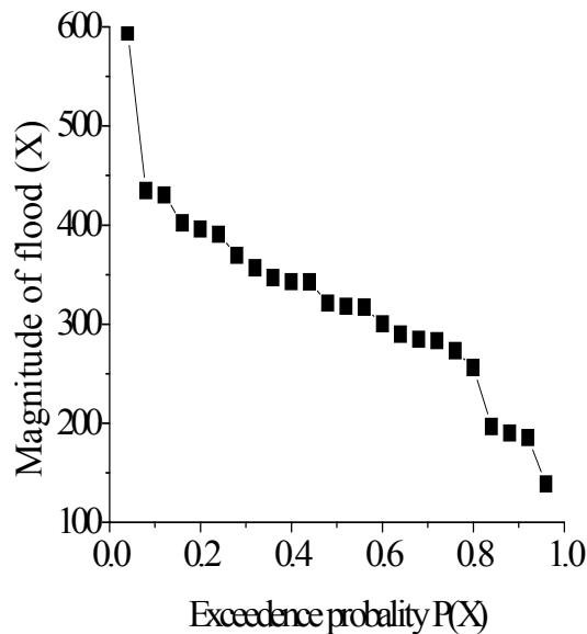
Figure 4. Magnitude of flood versus exceedance probability, black squared symbol represents flood magnitude corresponding to exceedance probabilities.
