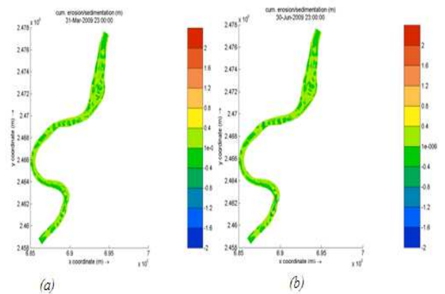
Figure 14. Cumulative erosion/deposition at the end of (a) March (b) June
