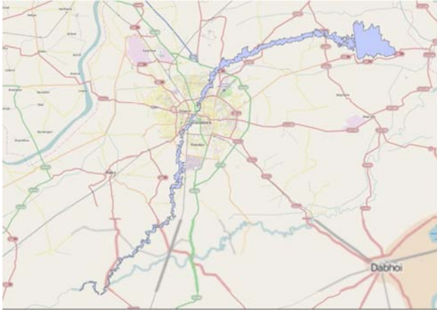
Figure 8. Floodplain map.
