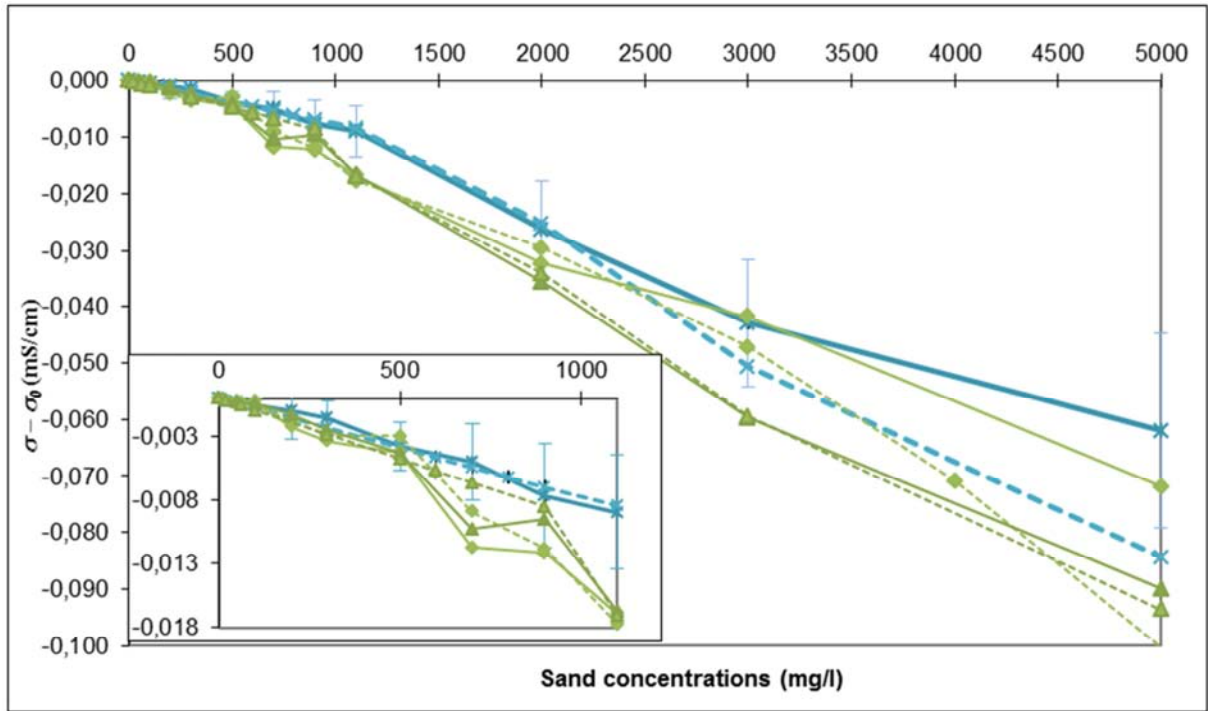
Figure 8. Conductivity differences measured (full lines) and obtained with equations (16) and (17) (Dashed lines) for the salinity S_p = 35 . Blue cross, 'desalted' sand, green diamonds and triangles, series 1 and 2 with 'natural' sand.
