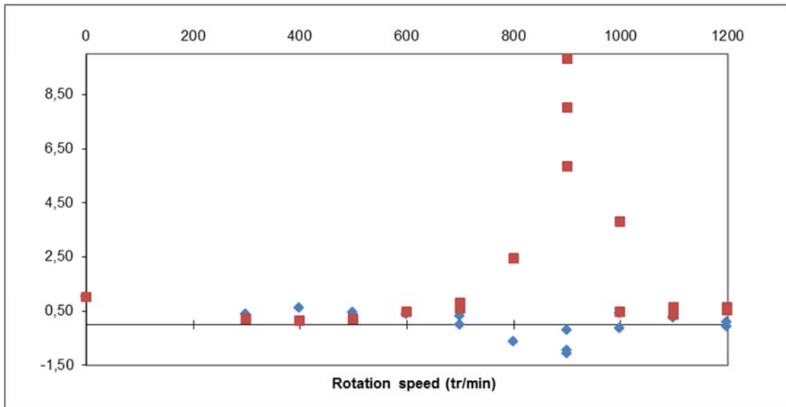
Figure 6. Red squares, ratio of the standard deviation of measurements series for a concentration of 500 \text{ mg l}^{-1} for different rotation speeds of the propeller from 0 to 1200 \text{ tr}\cdot\text{min}^{-1} , to the standard deviation at the null speed. Blue diamond, ratio of the average deviations of measurement series to the deviation at the null speed. The optimal speed is 900 \text{ tr}\cdot\text{min}^{-1} .
