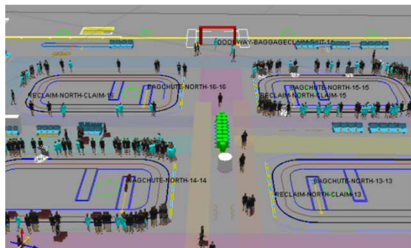
Figure 3. Terminal building internal process simulation.
