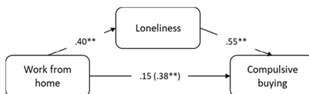
Figure 2. Hypothesis testing results.
