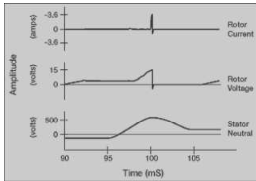
Fig 1. Time-Vs-Amplitude [4].
