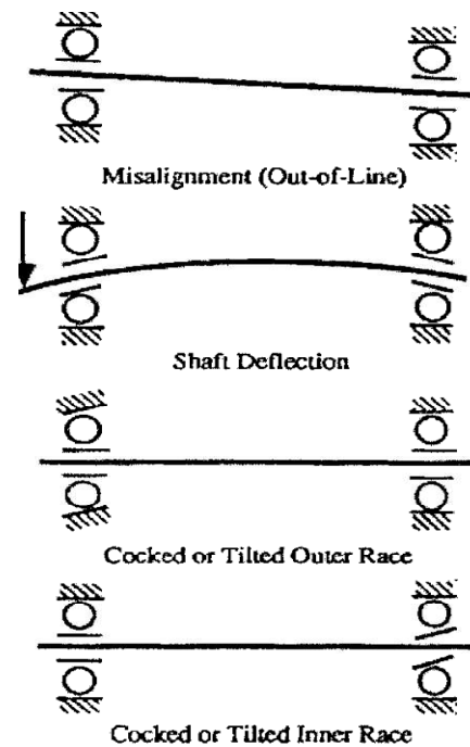
Fig 2. Four types of rolling-bearing misalignment [5].
