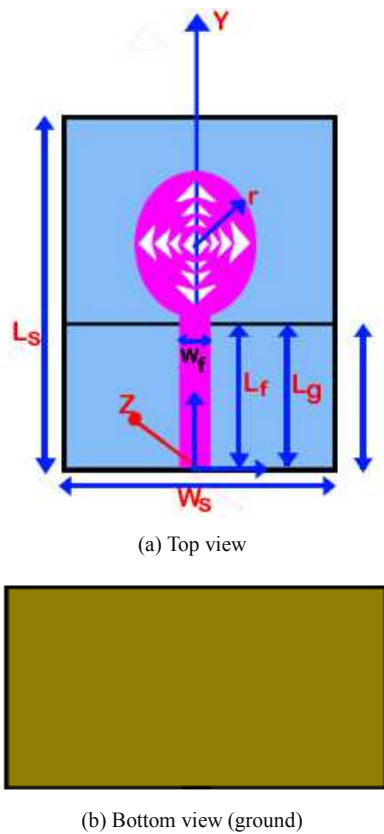
Figure 1. Geometry of proposed microstrip fed monopole antenna.
