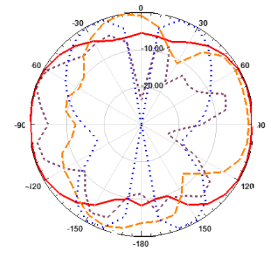
Figure 9. Radiation patterns at various frequencies of the antenna shown in Figure 1. Red (solid): H-Co. Poln.; Orange (Long-Dash): E-Co. Poln.; Blue (Dotted): E-Cross Poln.; Brown (Short-Dash): H-Cross Poln.
