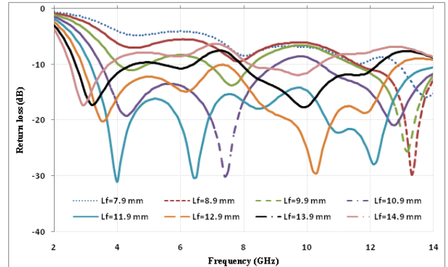
Figure 5. Return loss vs. frequency plot for feed length variation.
