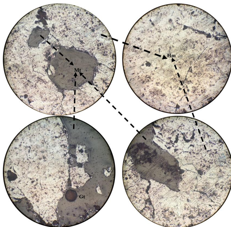
Figure 3. Micro photographs of soka iron ore samples (mineral compositions of mt =magnetite intruded to the hematite, hm= hematite and gt= goethite oolitic altered).
