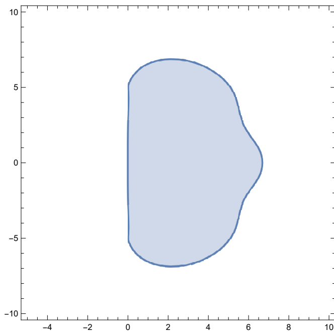
Figure 1. Region of absolute stability of One-step Method.
