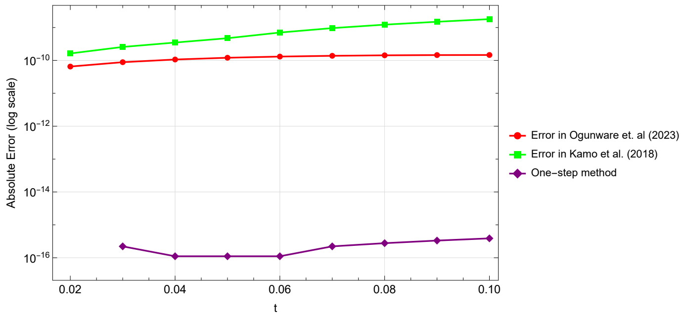
Figure 3. Comparison of results of example 3
