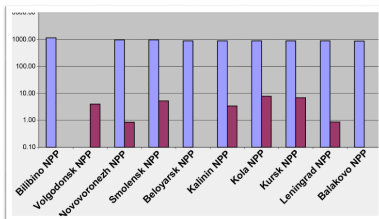
Figure 1. The natural radioactive background at the NPP localizations and the conservative predicted effective doses of irradiation for the “fishers” critical group of population on Russian Federation territory.
